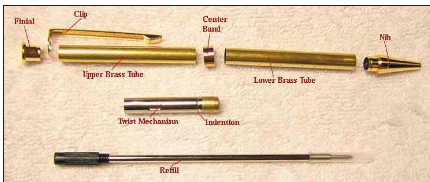
Parts diagram for 7mm pen.
